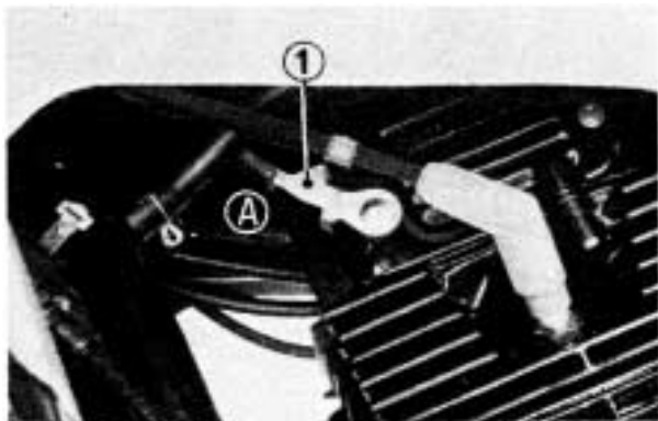
(1) Decompressor lever
