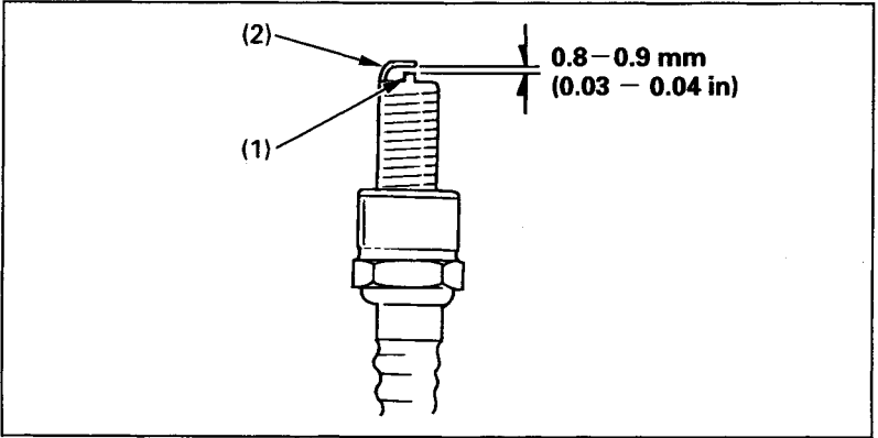
Fig. 4-15 (1) Center electrode (2) Side electrode
