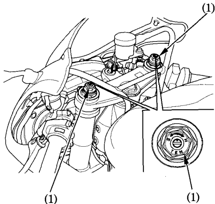
(1) Preload adjuster
