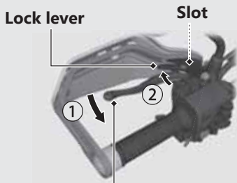
Parking brake lever
