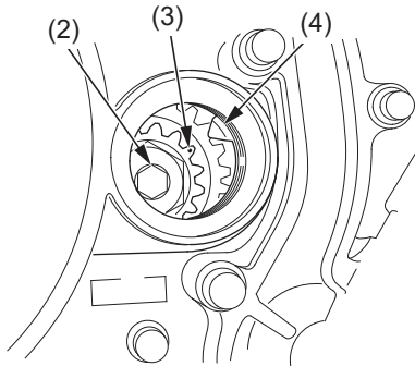
(2) primary drive gear bolt (3) punch mark (4) index mark
