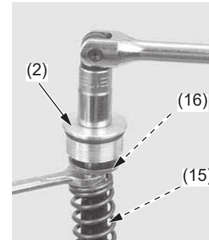
(2) fork cap (14) adjuster needle rod (15) piston rod
