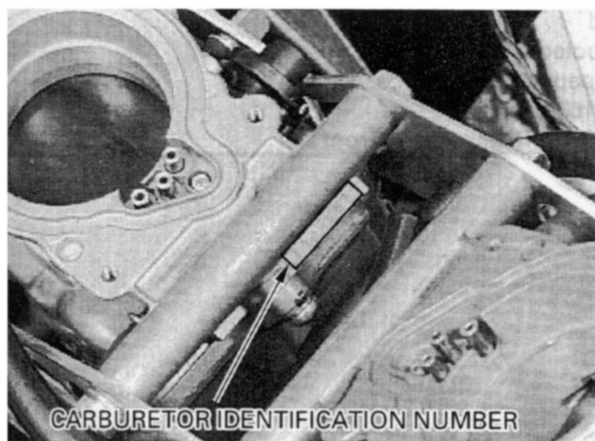
The carburetor identification number is stamped on the intake side of the carburetor body.
